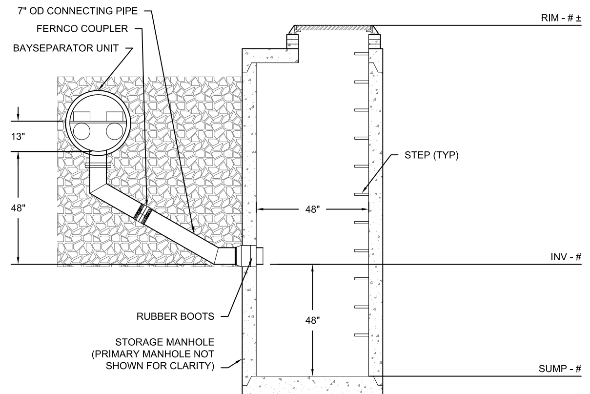
PROFILE B-B
