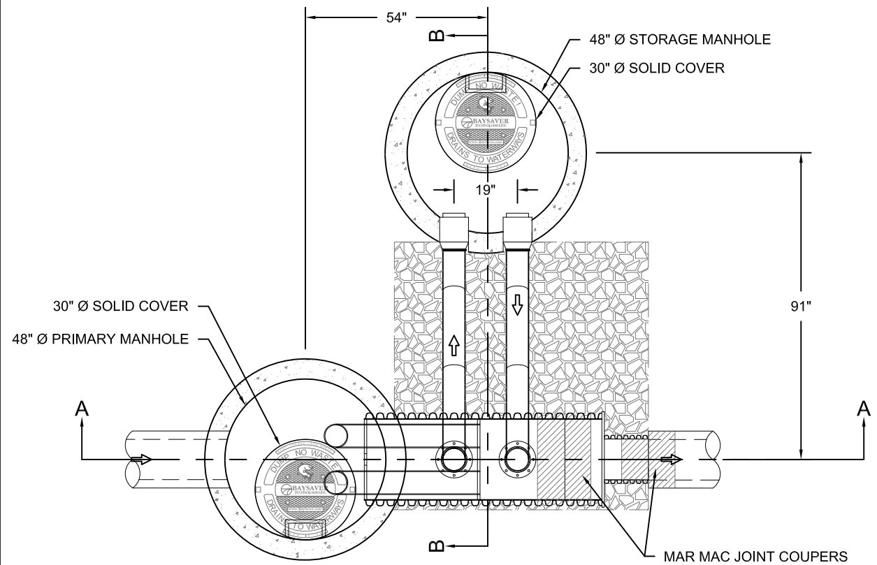
BAYSAVER BAYSEPARATOR 1K LEFT HAND UNIT
