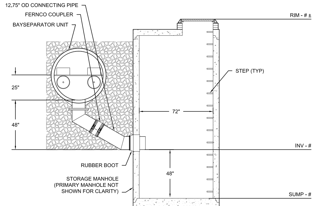
PROFILE B-B
