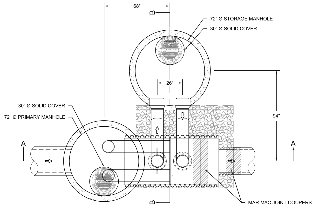
BAYSAVER BAYSEPARATOR 5K LEFT HAND UNIT
