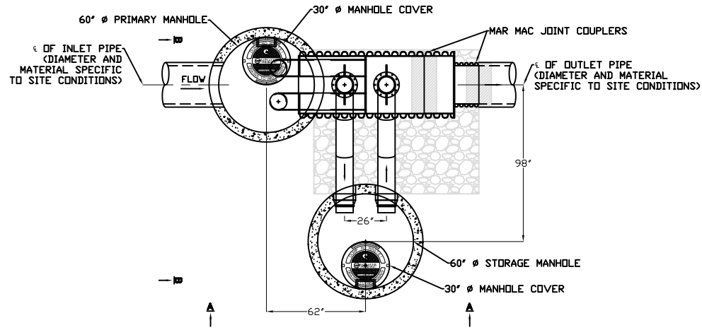
PLAN VIEW-BAYSAVER SEPARATION SYSTEM (RIGHT HAND ORIENTATION SHOWN)
