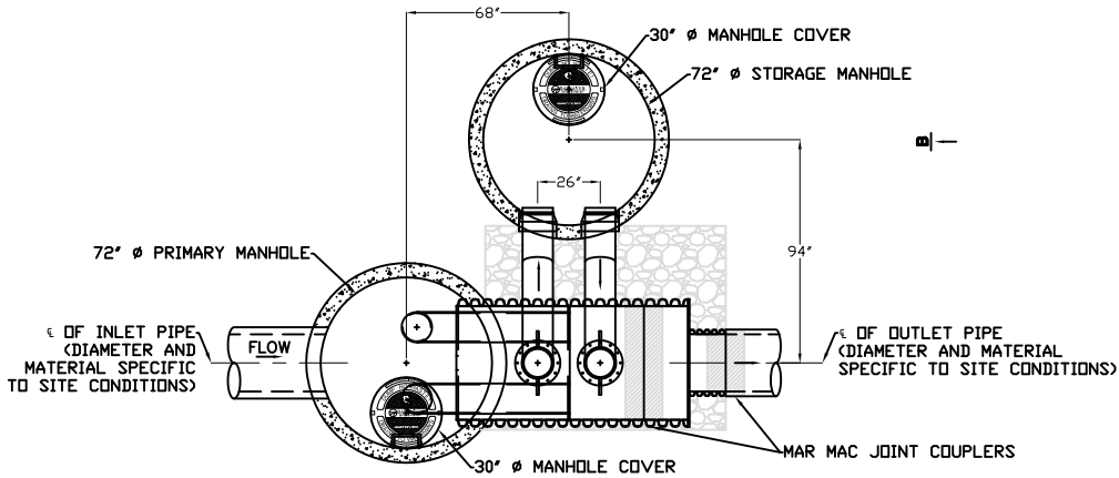
PLAN VIEW-BAYSAVER SEPARATION SYSTEM (LEFT HAND ORIENTATION SHOWN)
