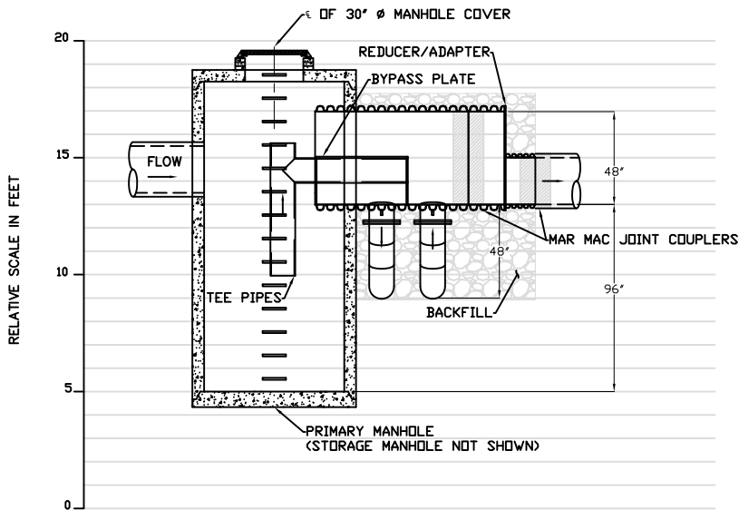
PROFILE VIEW A-A
